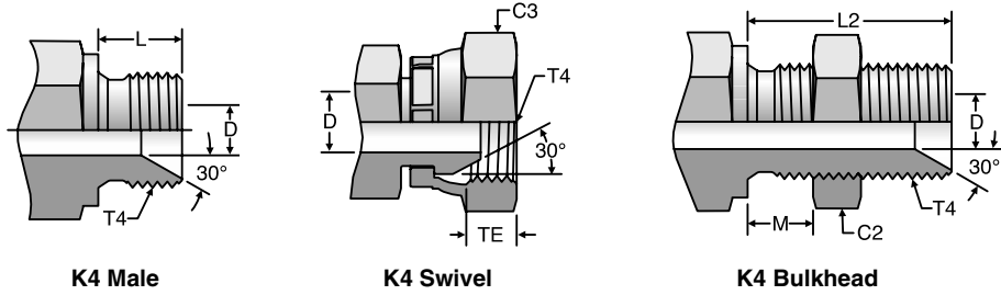
K4 Male K4 Swivel K4 Bulkhead
